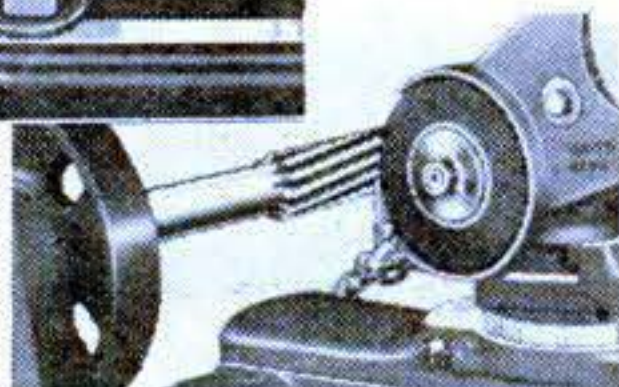
Above: Grinding a cutter with spring stop in holding fixture. Right: Grinding spiral reamer.
